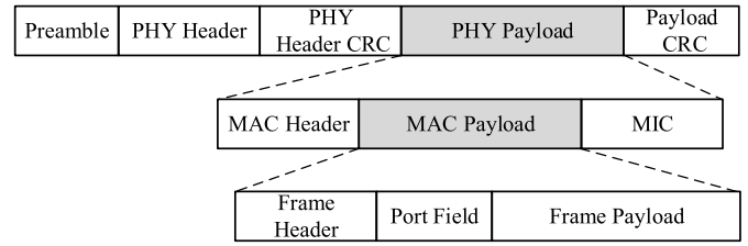
Fig. 17. The structure of LoRa frame.
